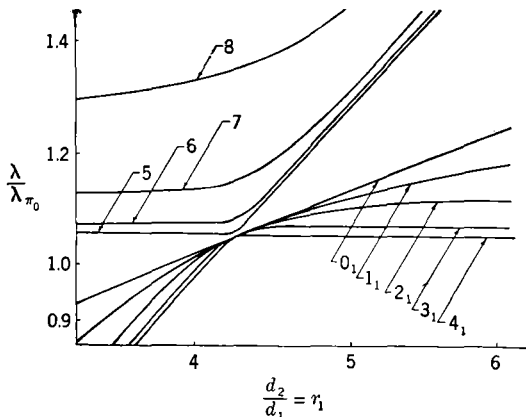
FIG. 3-4.—Mode spectrum, for large values of r_1 , of the rising-sun system of Fig. 3-3. The two groups shown correspond to the first group of the small-resonator system and the second group of the large-resonator system.
